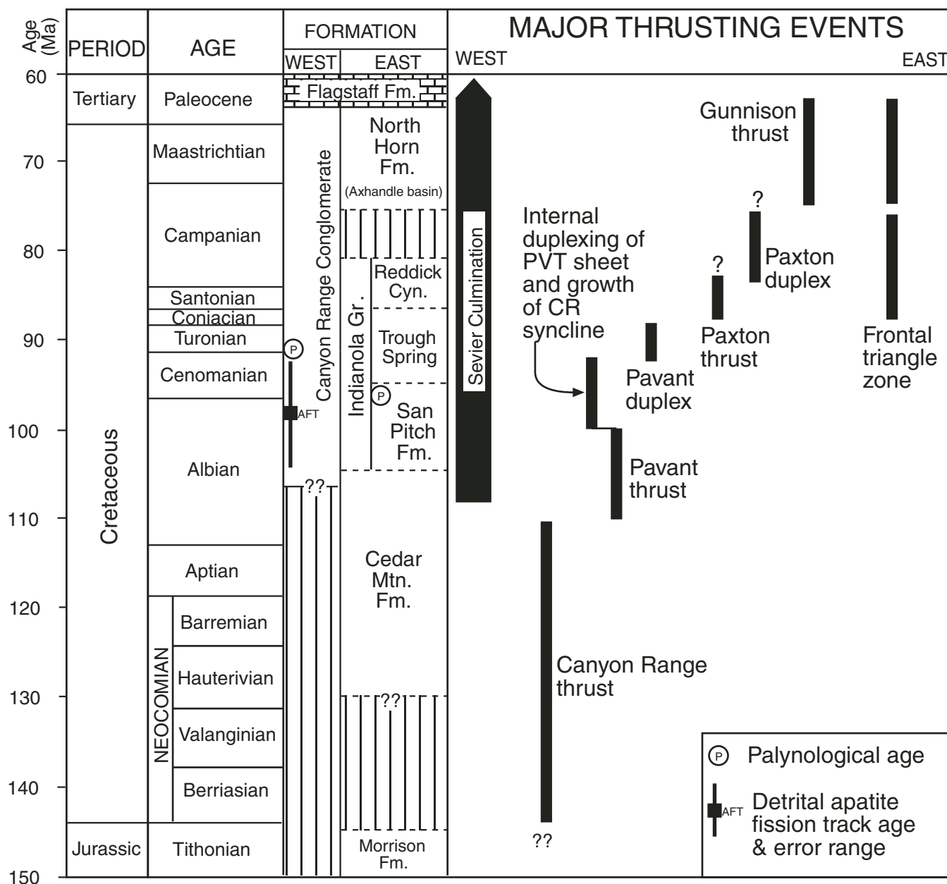
Figure 10. Chart showing the timing of major thrusting events and growth of the Sevier culmination in the central Utah segment of the Sevier fold-and-thrust belt. CR—Canyon Range; PVT—Pavant thrust.
